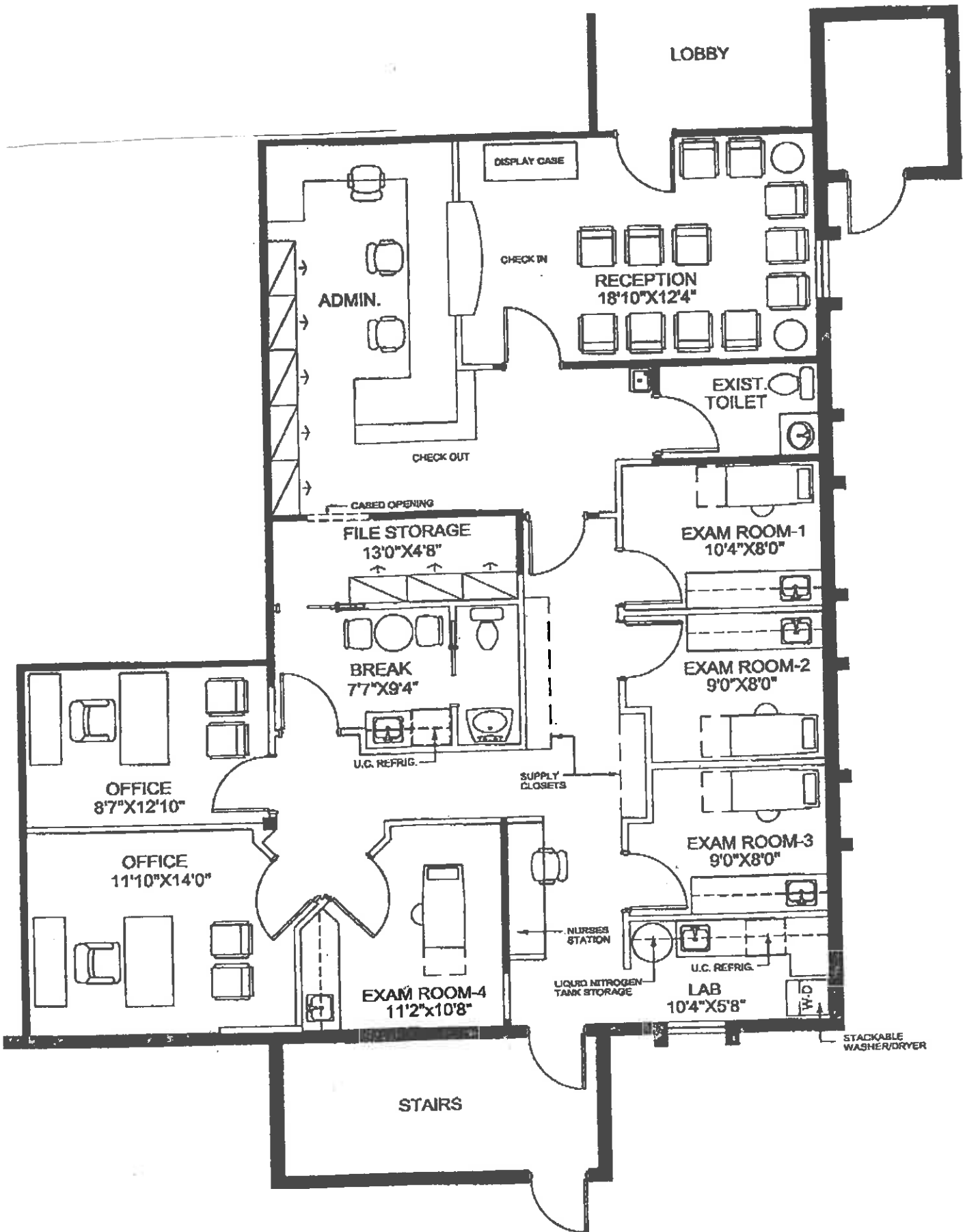
FLOOR PLAN 1/4" = 1'-0"
